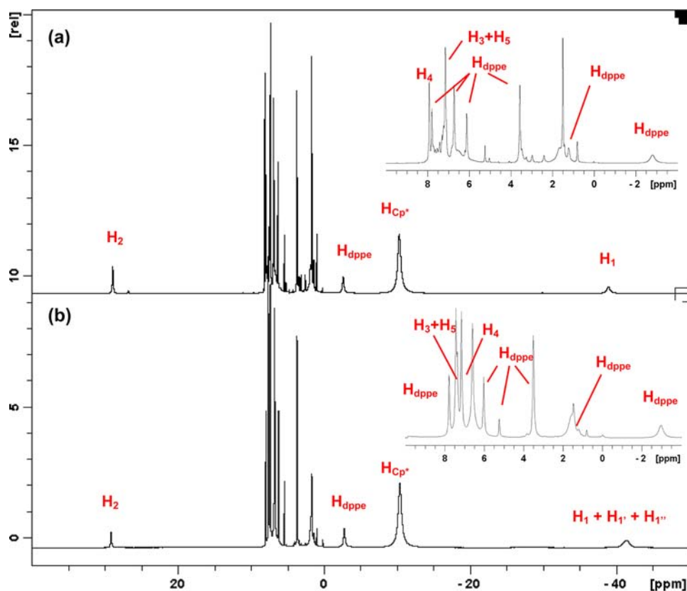
Figure 3. ^1\text{H} NMR spectra of 1 [\text{PF}_6] (a) and 2 [\text{PF}_6] (b) in \text{CD}_2\text{Cl}_2 at 25^\circ\text{C} with proposed assignment according to Chart 1 for selected protons. Specific assignment of protons in the diamagnetic range are given on scaled up spectra. Unlabeled signals correspond to residual solvent peaks.
